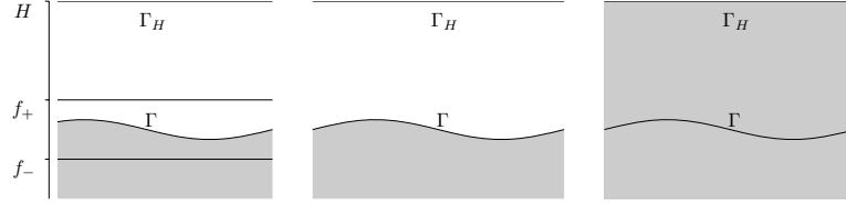
FIGURE 1. The domain for the boundary value problem.
